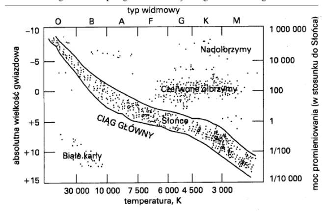
Diagram Hertzsprunga - Russela
